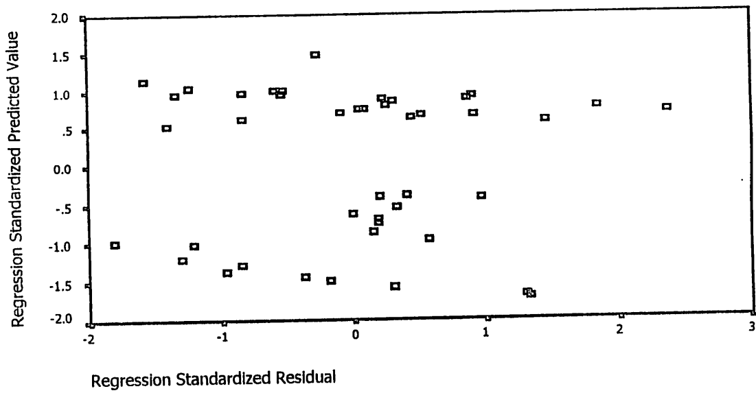
Scatterplot Dependent Variable: Y
