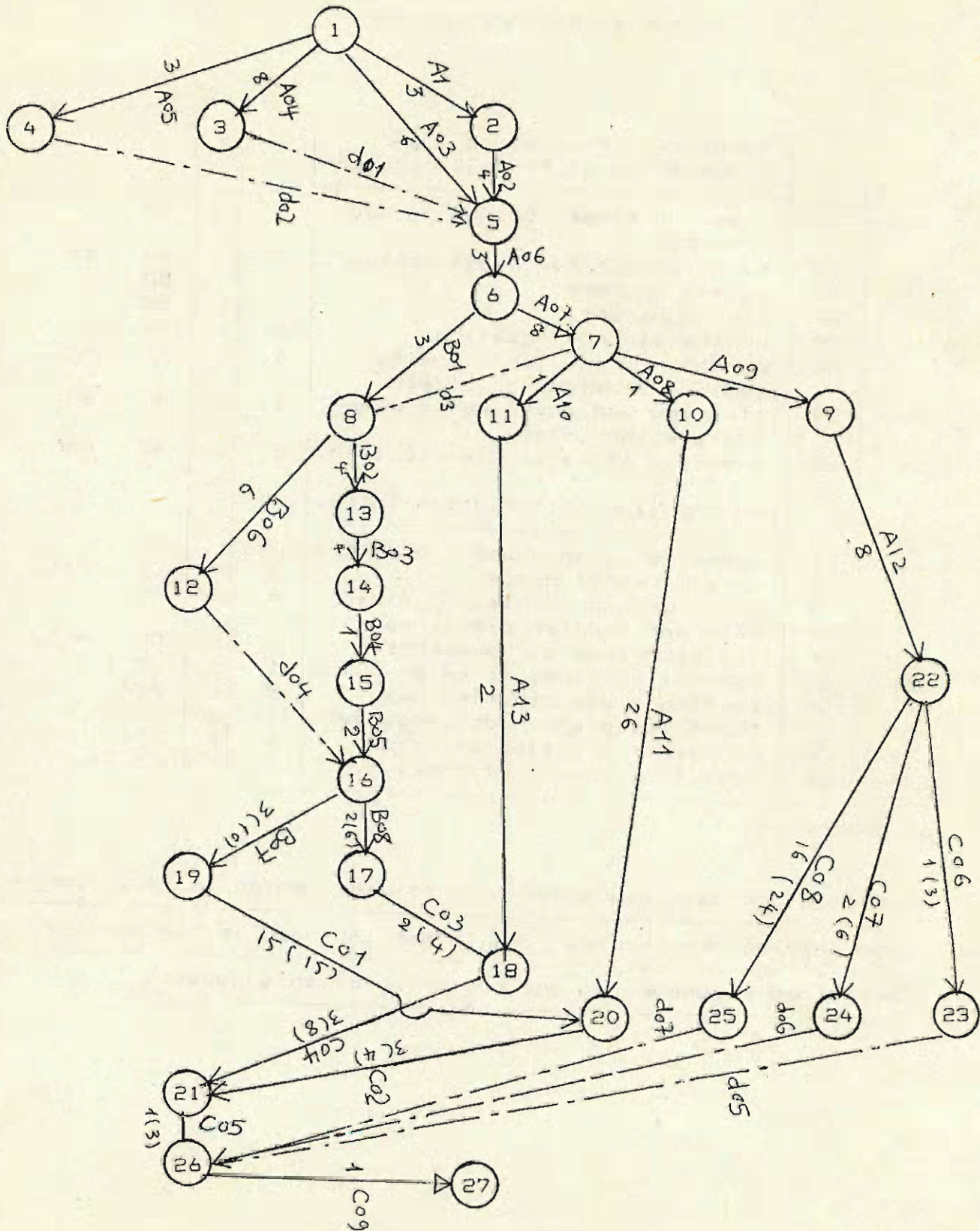
The Activity-On-Arrow Network :
